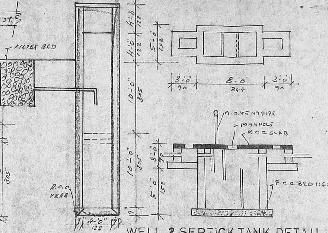
WELL & SEPTICK TANK DETAIL
