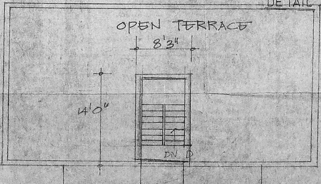
TERRACE PLAN
